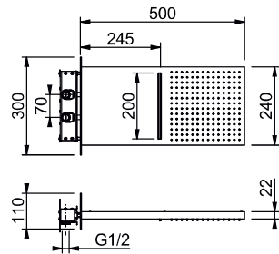
DIFUSOR 240 MM
