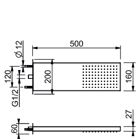
DIFUSOR 160 MM
