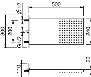
DIFUSOR 240 MM
