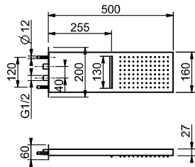
DIFUSOR 160 MM
